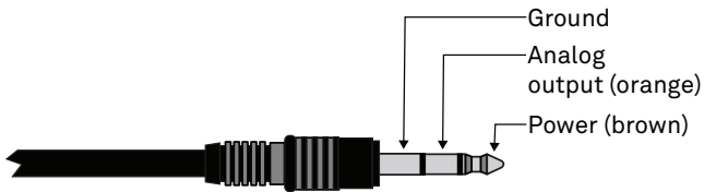
Figure 1 Stereo plug connector
